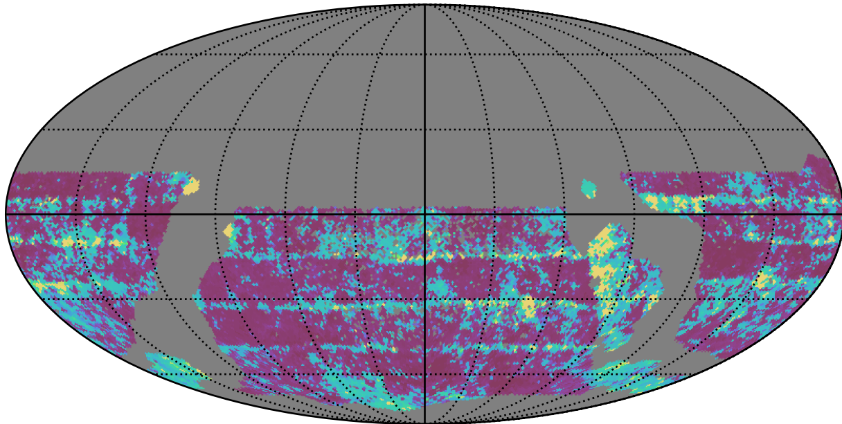
scp_reweight_v3.3_10yrs WFD z band: 20thPercentile Inter-Night Gap
