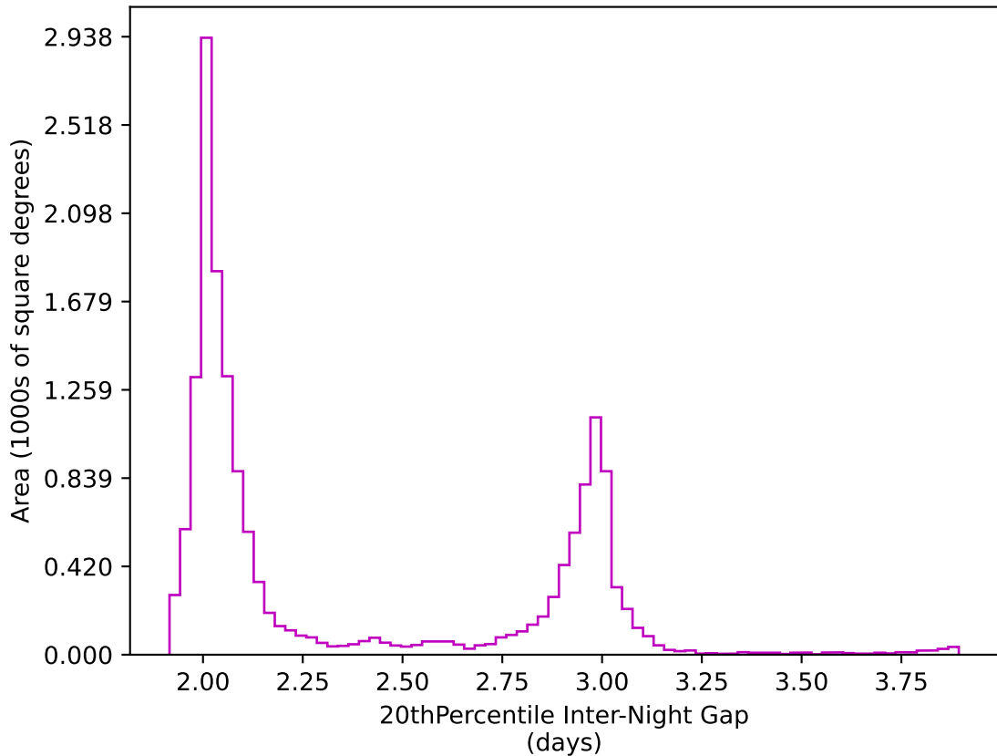
scp_reweight_v3.3_10yrs WFD z band: 20thPercentile Inter-Night Gap
