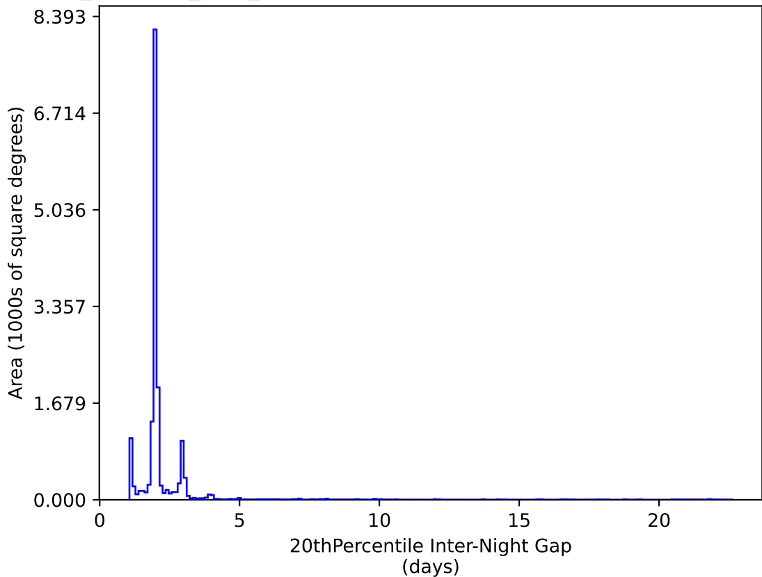
scp_reweight_v3.3_10yrs WFD y band: 20thPercentile Inter-Night Gap
