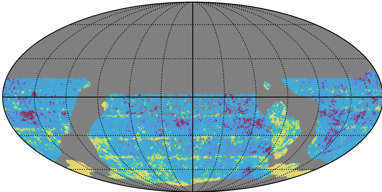
scp_reweight_v3.3_10yrs WFD r band: 20thPercentile Inter-Night Gap
