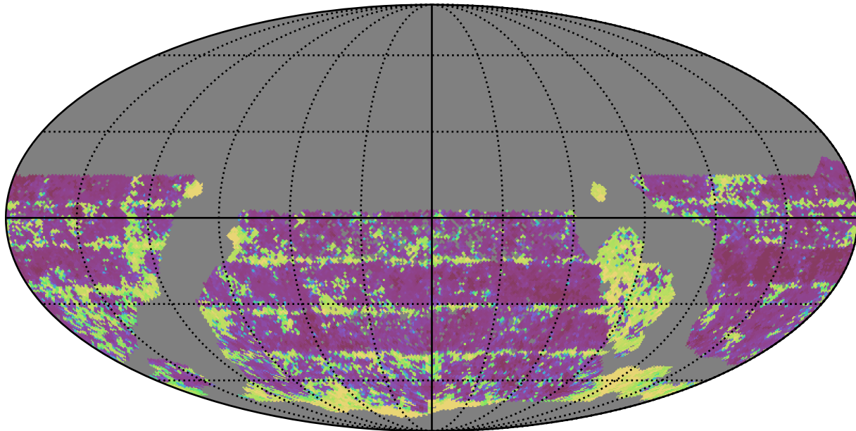
scp_reweight_v3.3_10yrs WFD i band: 20thPercentile Inter-Night Gap
