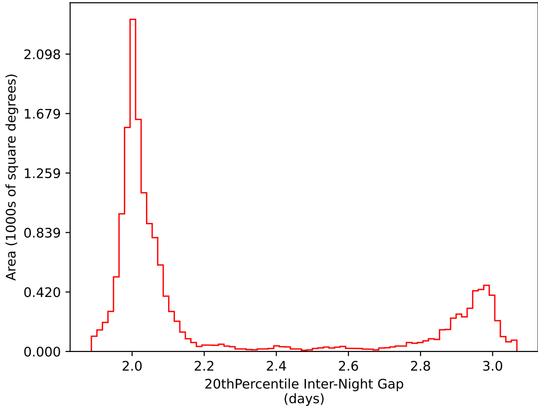
scp_reweight_v3.3_10yrs WFD i band: 20thPercentile Inter-Night Gap
