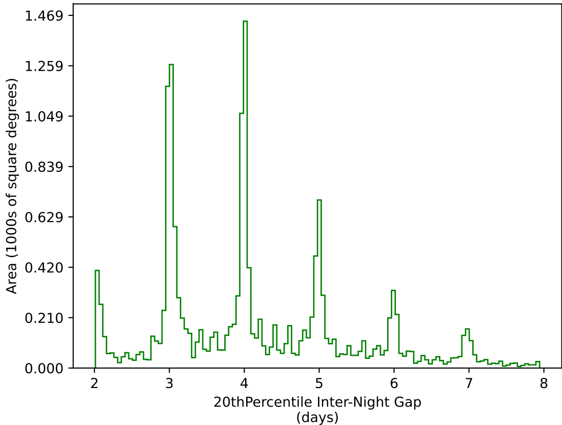
scp_reweight_v3.3_10yrs WFD g band: 20thPercentile Inter-Night Gap
