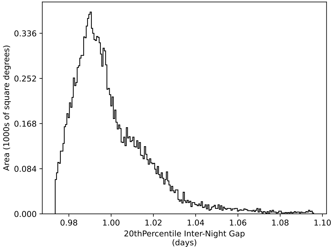
scp_reweight_v3.3_10yrs WFD all bands: 20thPercentile Inter-Night Gap
