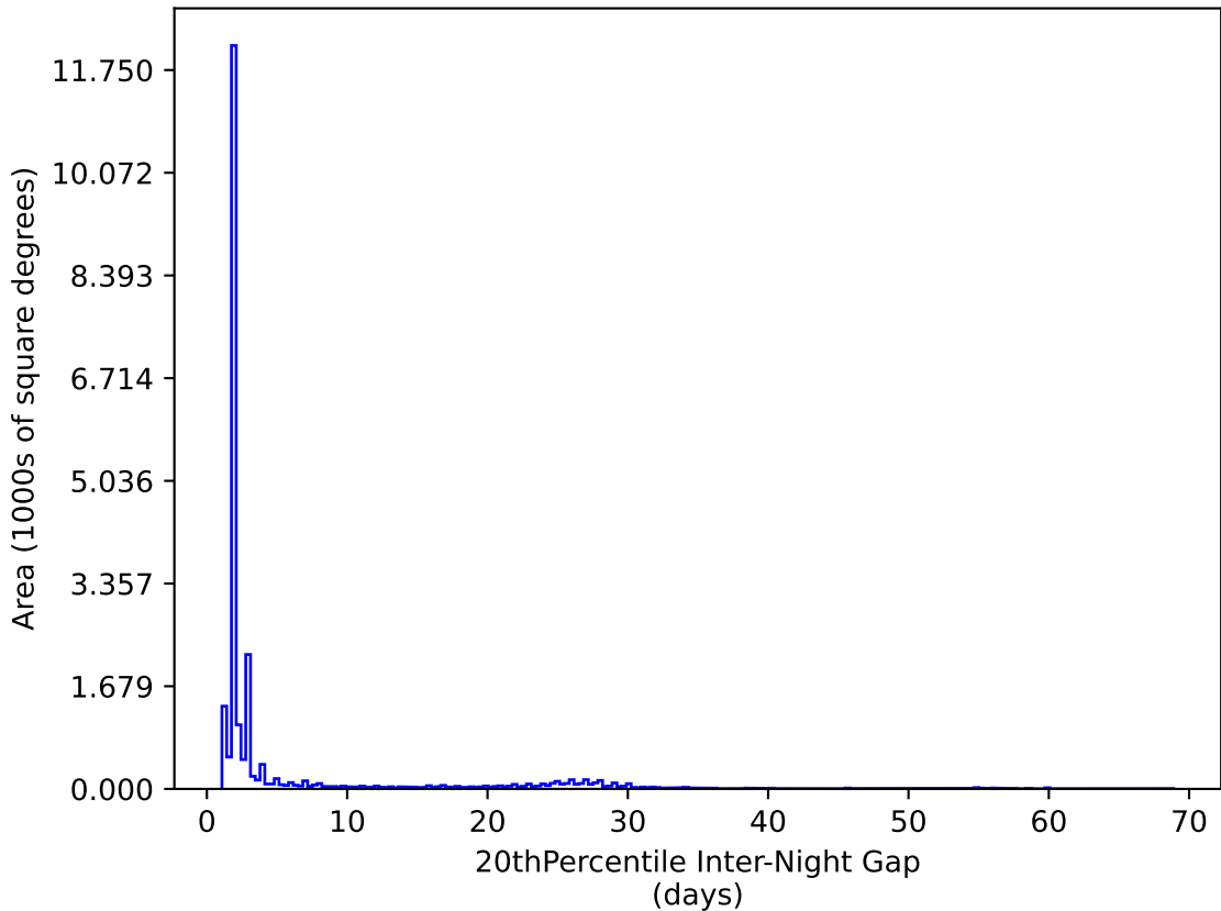
scp_reweight_v3.3_10yrs All sky y band: 20thPercentile Inter-Night Gap
