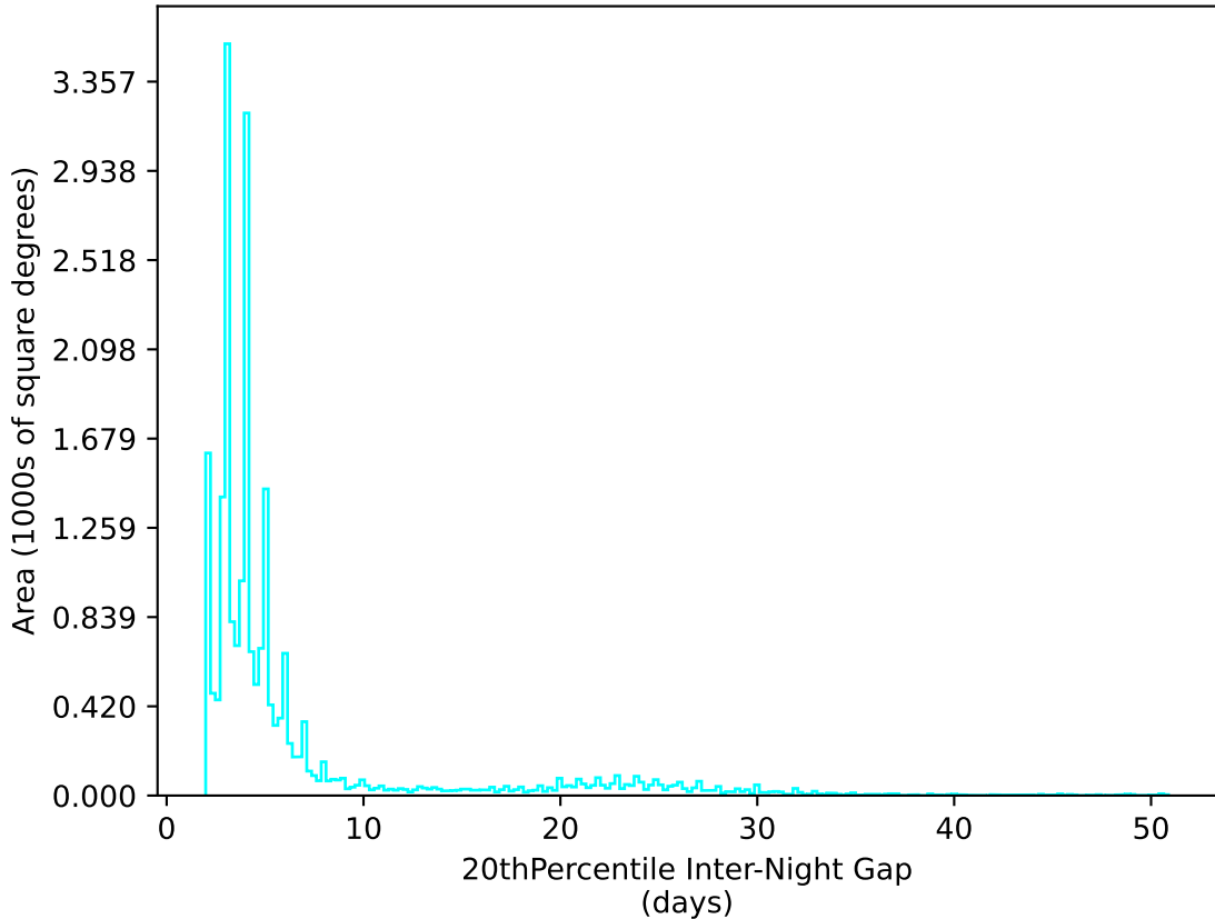
scp_reweight_v3.3_10yrs All sky u band: 20thPercentile Inter-Night Gap
