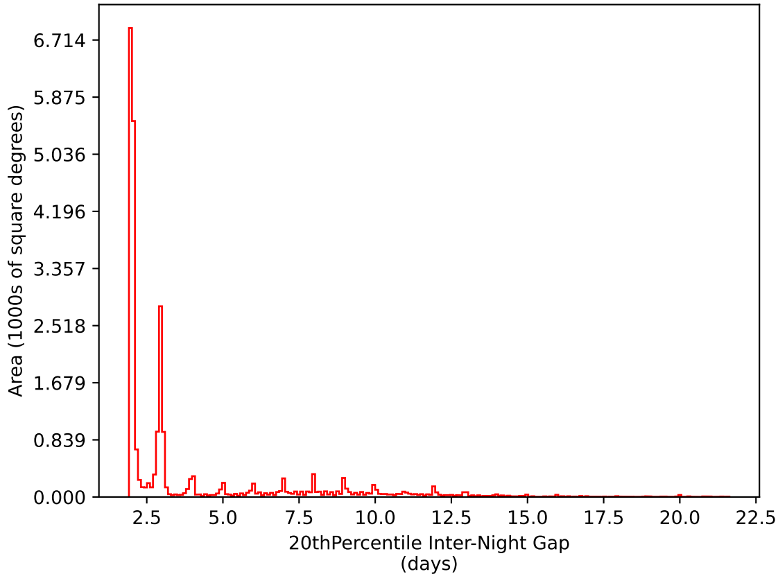
scp_reweight_v3.3_10yrs All sky i band: 20thPercentile Inter-Night Gap
