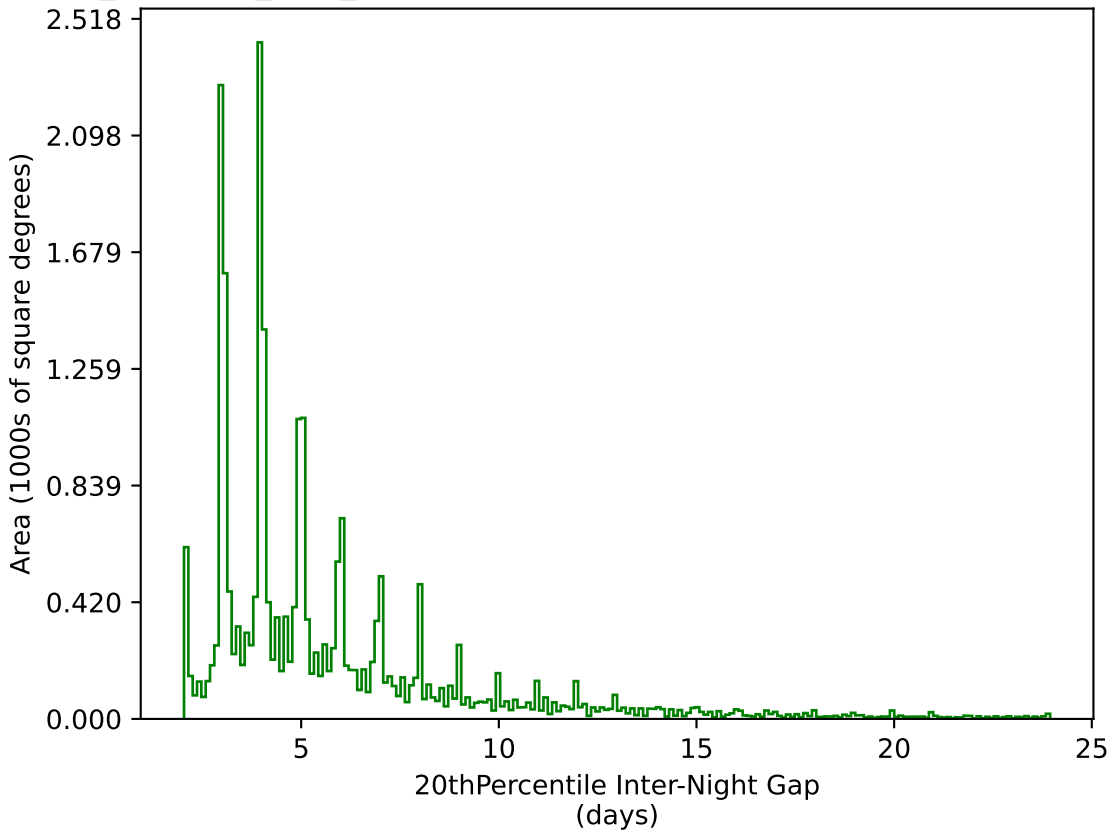
scp_reweight_v3.3_10yrs All sky g band: 20thPercentile Inter-Night Gap
