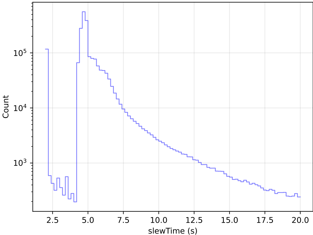
scp_reweight_v3.3_10yrs All visits: Zoom Slew Time Histogram
