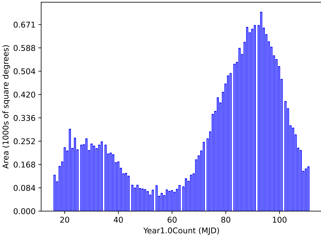
scp_reweight_v3.3_10yrs night < 365.25: Year1.0Count
