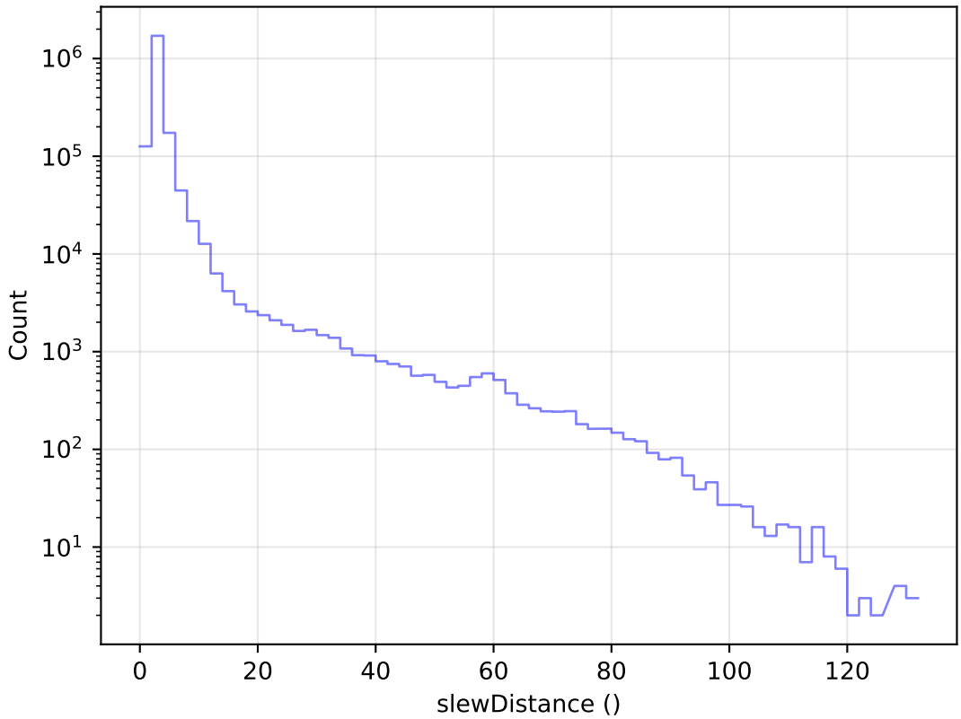
scp_reweight_v3.3_10yrs All visits: Slew Distance Histogram
