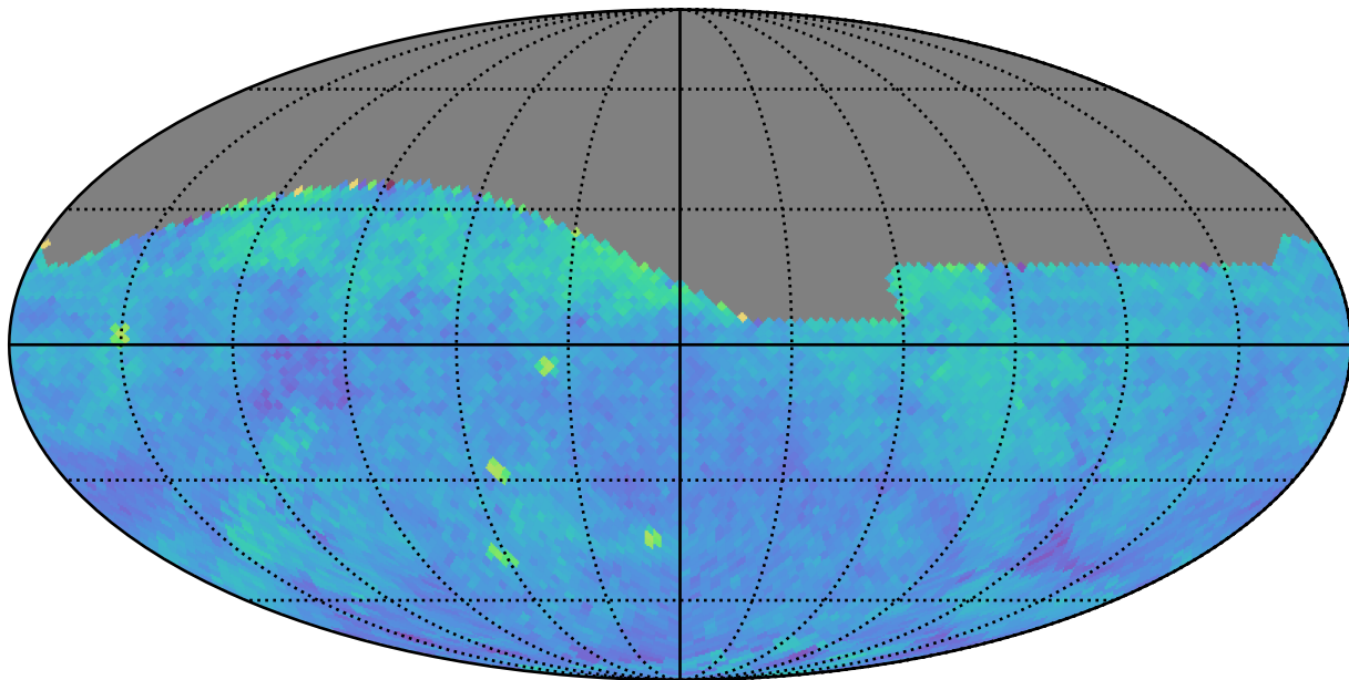
scp_reweight_v3.3_10yrs (g or r or i): PairFraction
