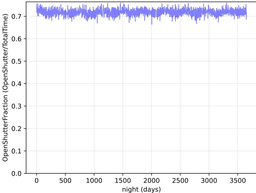
scp_reweight_v3.3_10yrs : OpenShutterFraction
