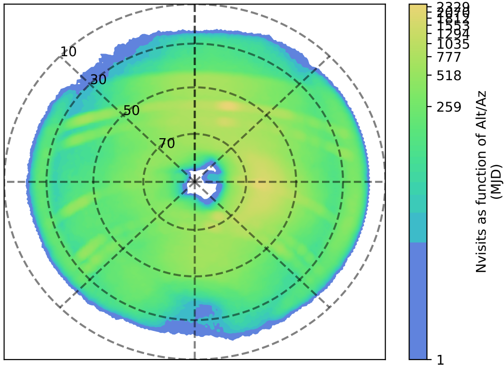
scp_reweight_v3.3_10yrs z: Nvisits as function of Alt/Az
