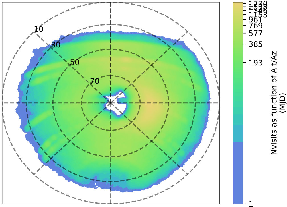
scp_reweight_v3.3_10yrs y: Nvisits as function of Alt/Az
