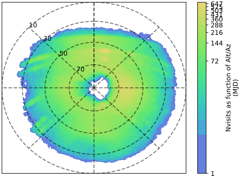
scp_reweight_v3.3_10yrs u: Nvisits as function of Alt/Az
