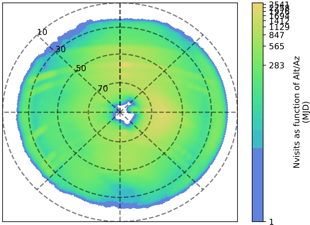
scp_reweight_v3.3_10yrs i: Nvisits as function of Alt/Az
