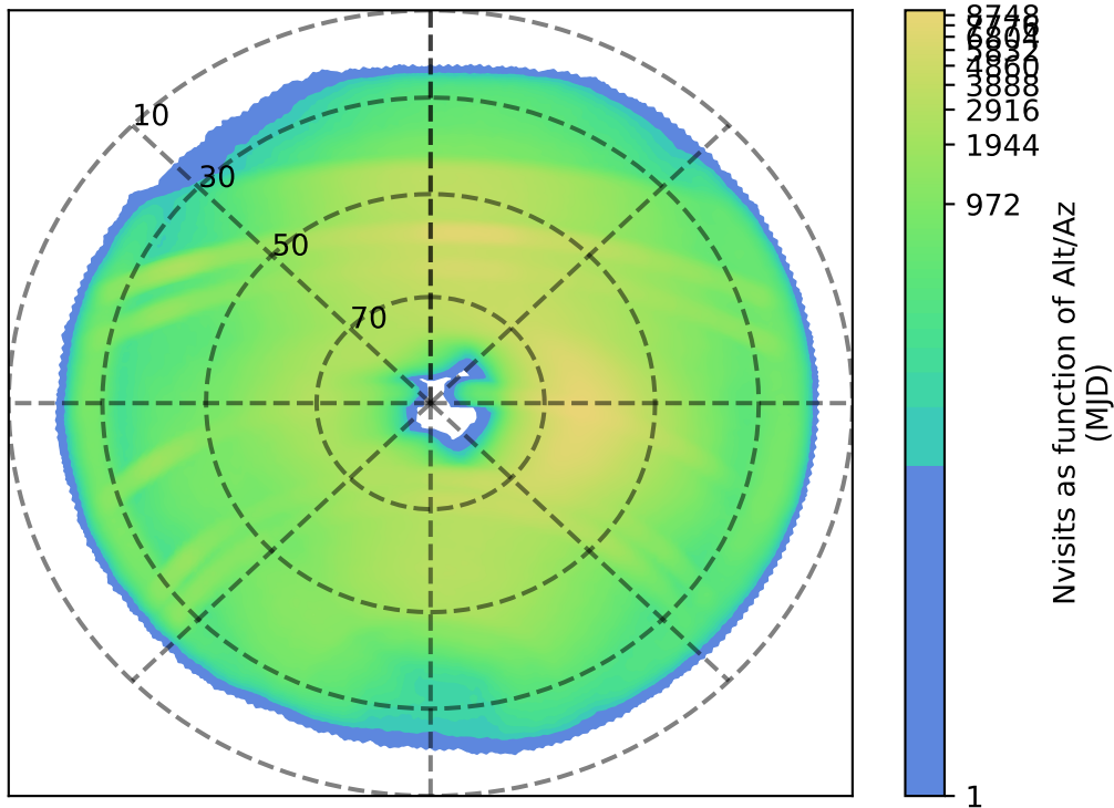
scp_reweight_v3.3_10yrs : Nvisits as function of Alt/Az
