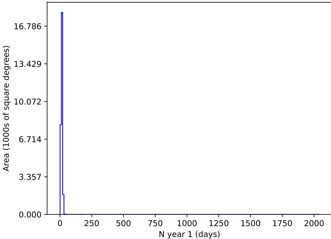
scp_reweight_v3.3_10yrs z and night < 365: N year 1
