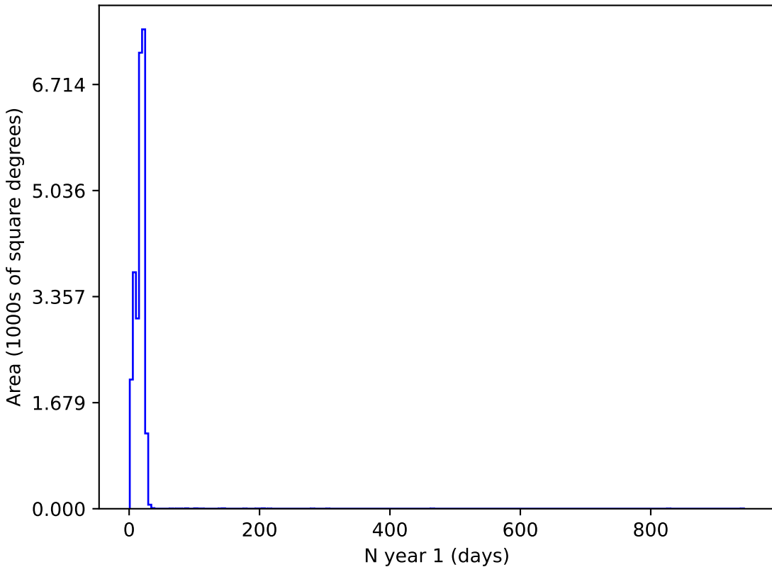
scp_reweight_v3.3_10yrs y and night < 365: N year 1
