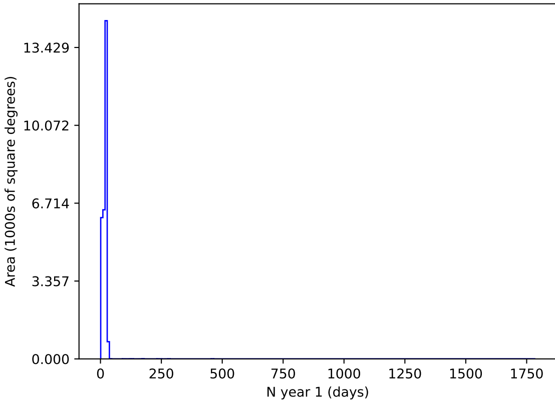
scp_reweight_v3.3_10yrs i and night < 365: N year 1
