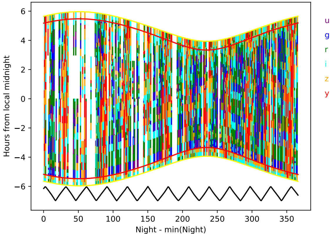
scp_reweight_v3.3_10yrs year 9-10: Hourglass
