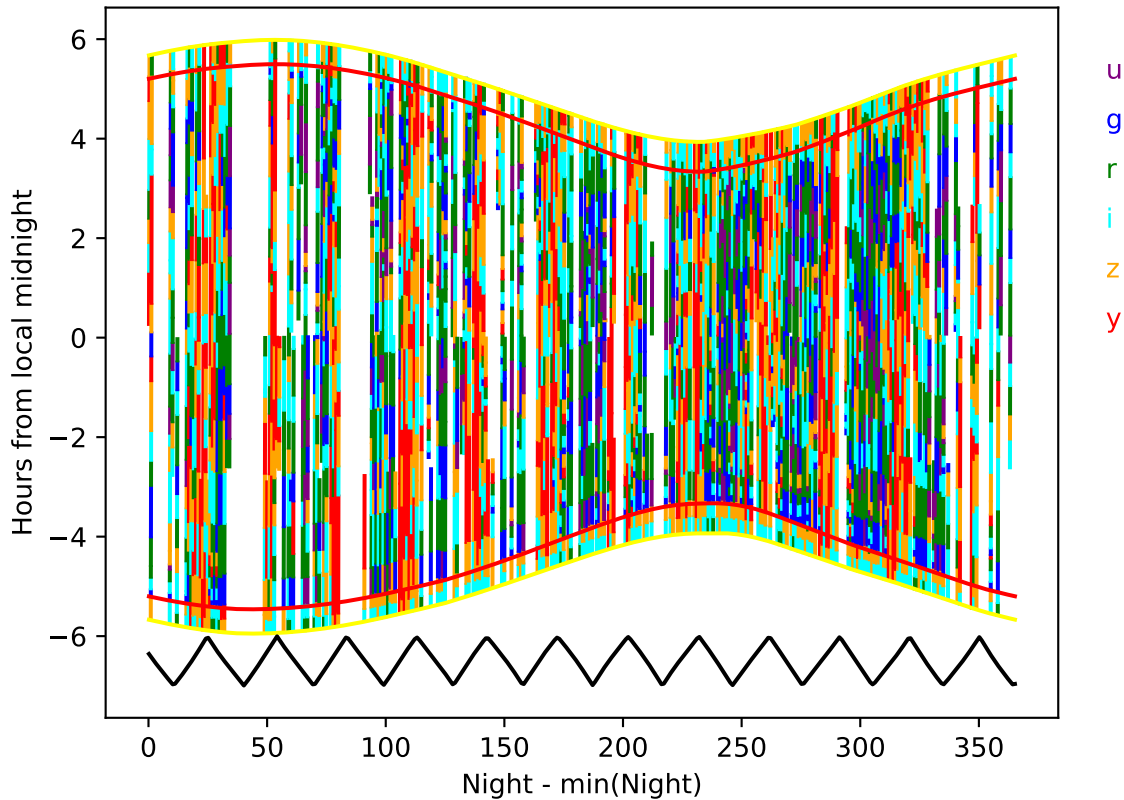
scp_reweight_v3.3_10yrs year 4-5: Hourglass
