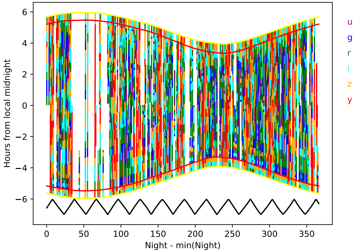
scp_reweight_v3.3_10yrs year 3-4: Hourglass
