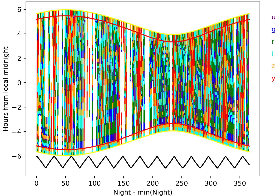
scp_reweight_v3.3_10yrs year 1-2: Hourglass
