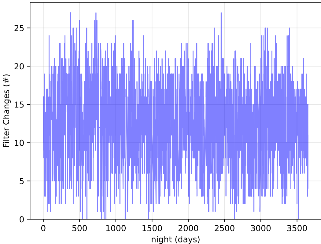
scp_reweight_v3.3_10yrs : Filter Changes
