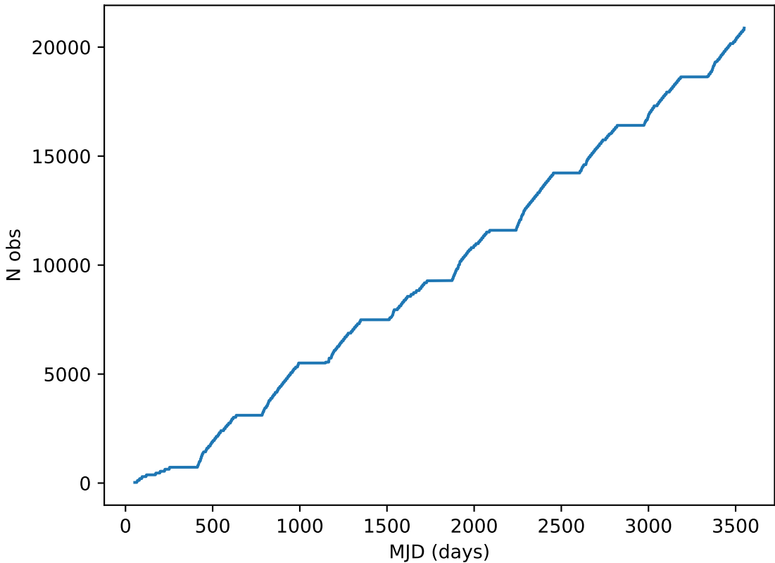
scp_reweight_v3.3_10yrs note like DD:ELAISS1%: Cumulative
