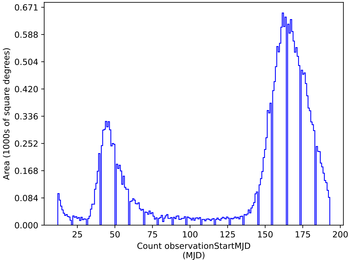
scp_reweight_v3.3_10yrs z: Count observationStartMJD
