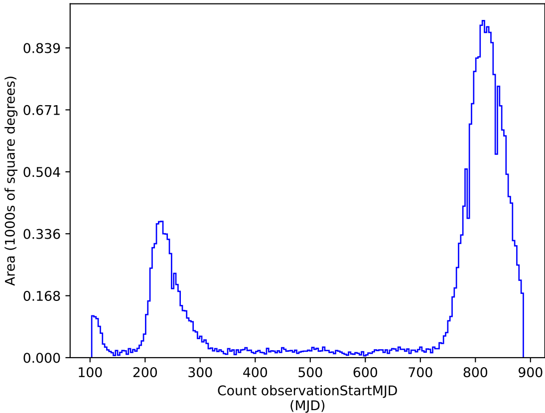
scp_reweight_v3.3_10yrs : Count observationStartMJD
