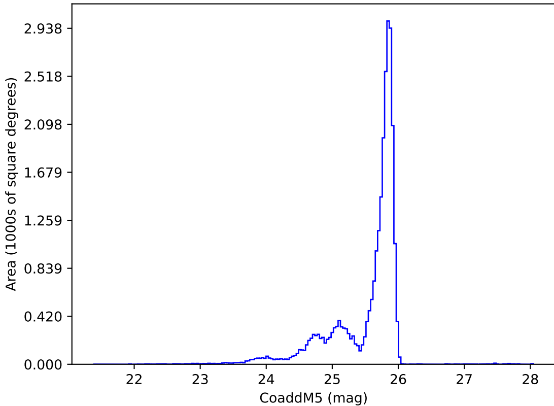
scp_reweight_v3.3_10yrs z: CoaddM5
