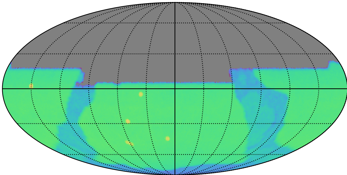
scp_reweight_v3.3_10yrs y: CoaddM5
