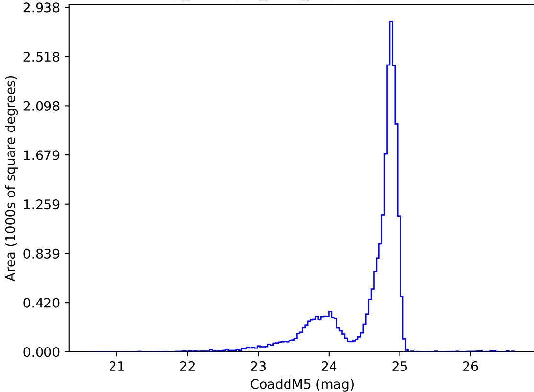
scp_reweight_v3.3_10yrs y: CoaddM5
