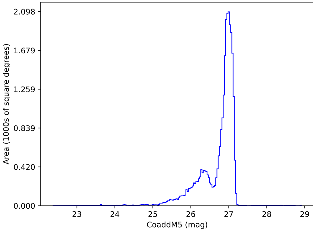
scp_reweight_v3.3_10yrs r: CoaddM5
