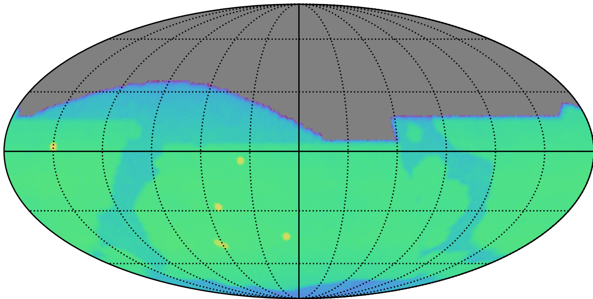
scp_reweight_v3.3_10yrs i: CoaddM5
