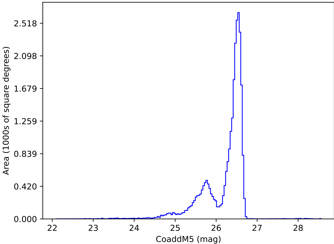
scp_reweight_v3.3_10yrs i: CoaddM5
