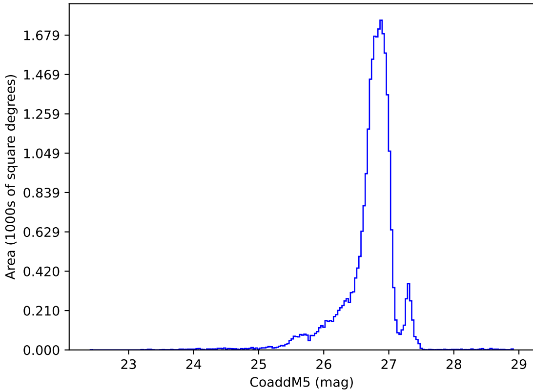
scp_reweight_v3.3_10yrs g: CoaddM5
