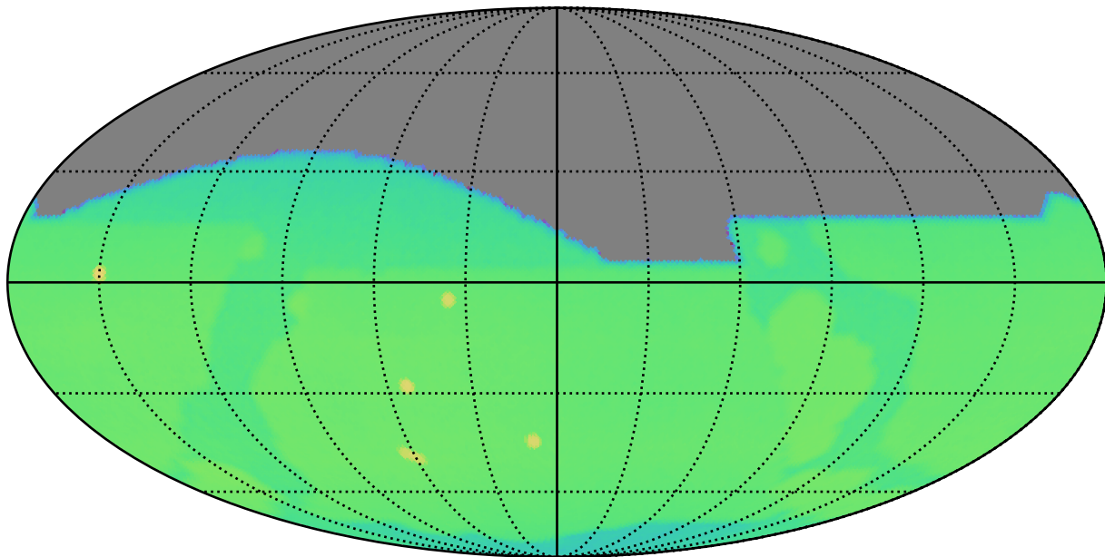
scp_reweight_v3.3_10yrs : CoaddM5
