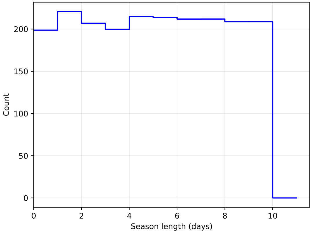
scp_reweight_v3.3_10yrs DD:ELAISS1 all bands: SeasonLength
