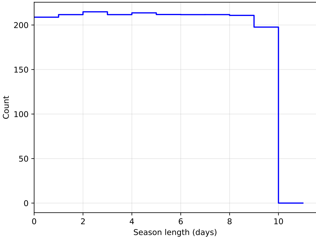
scp_reweight_v3.3_10yrs DD:EDFS all bands: SeasonLength
