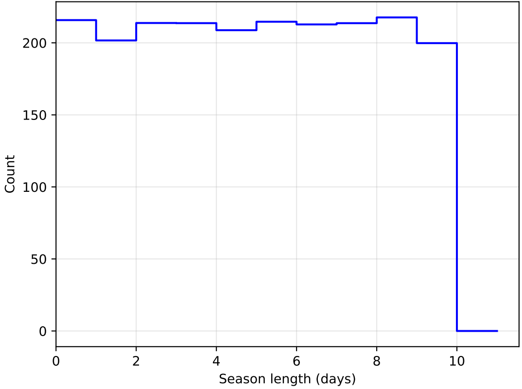
scp_reweight_v3.3_10yrs DD:ECDFS all bands: SeasonLength
