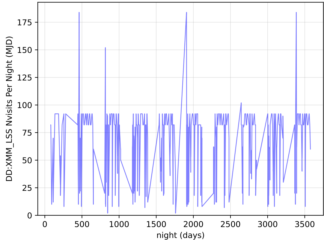
scp_reweight_v3.3_10yrs all bands: DD:XMM_LSS Nvisits Per Night
