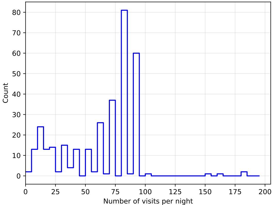
scp_reweight_v3.3_10yrs all bands: DD:XMM_LSS NVisitsPerNight
