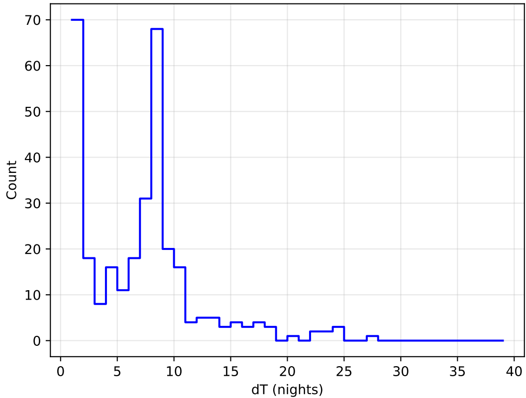
scp_reweight_v3.3_10yrs all bands: DD:XMM_LSS Delta Nights Histogram
