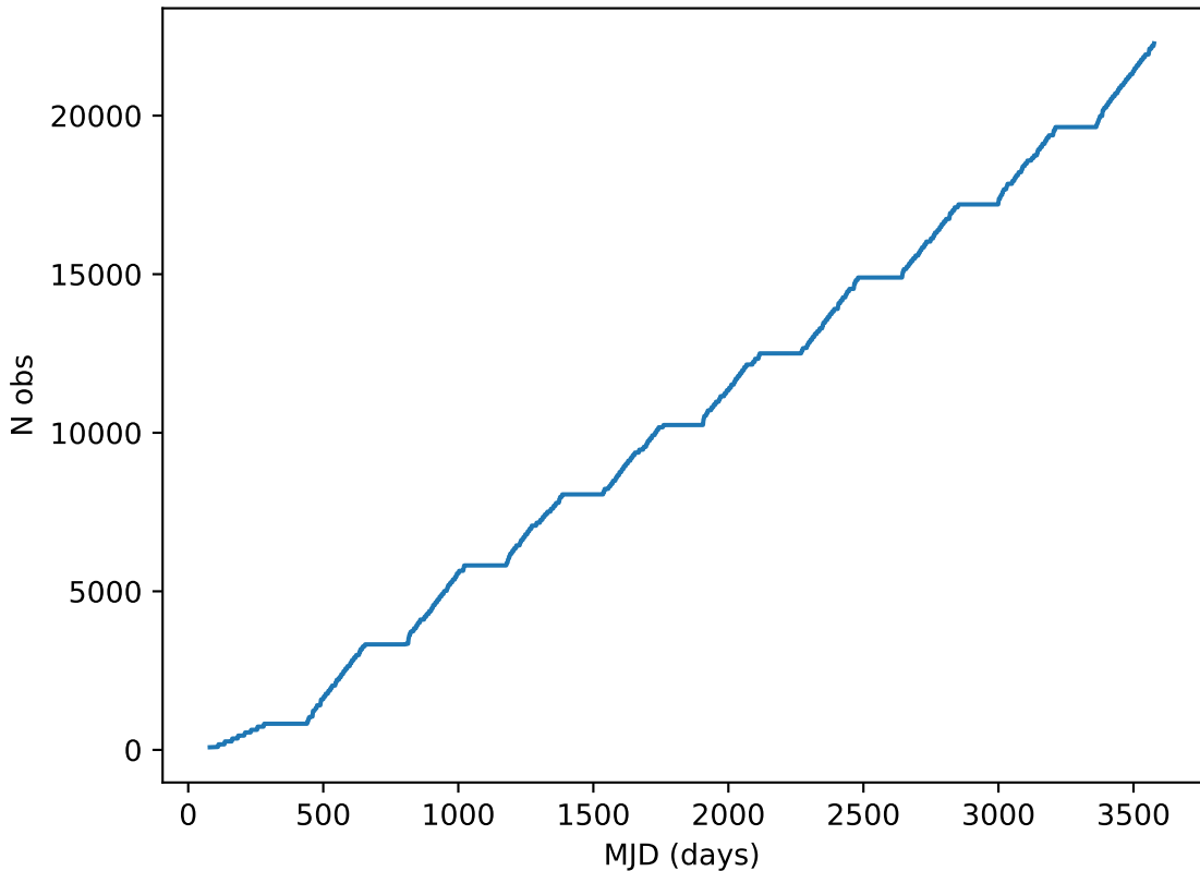
scp_reweight_v3.3_10yrs all bands: DD:XMM_LSS Cumulative NVisits
