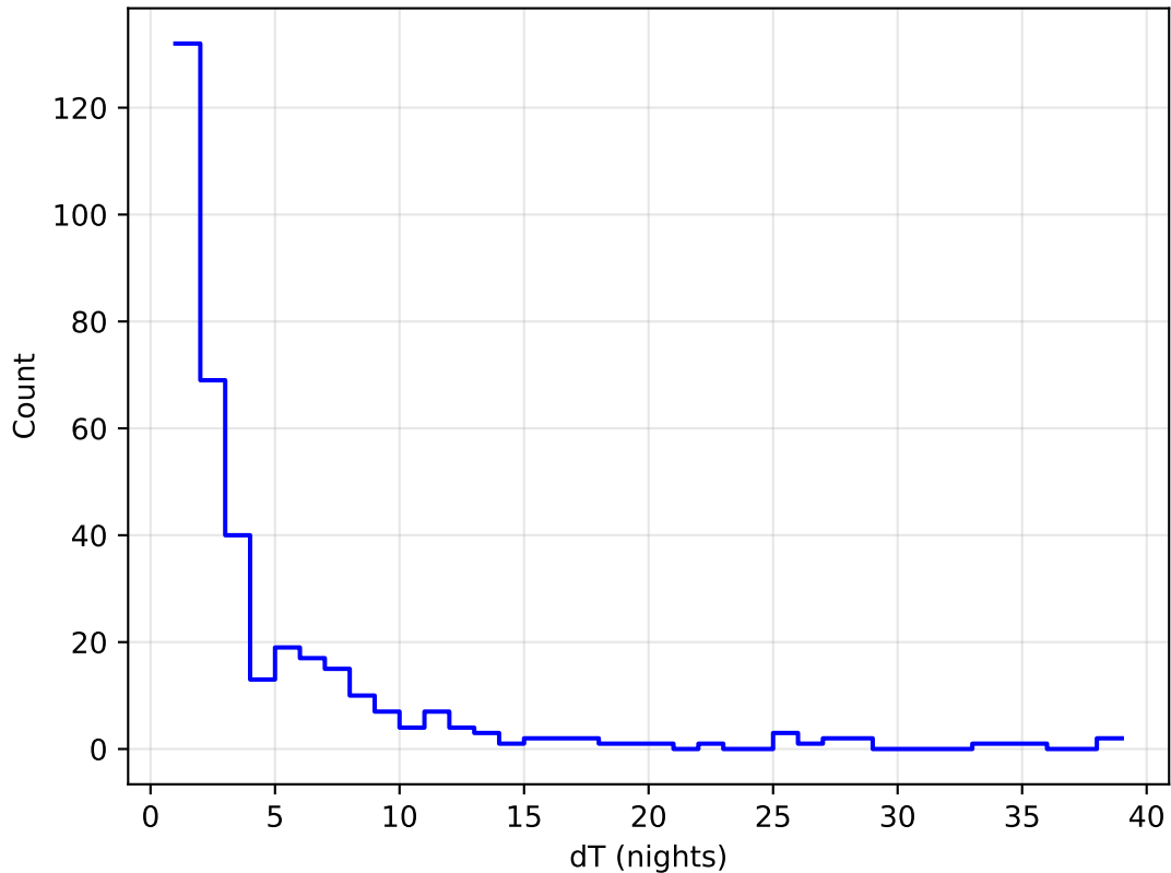
scp_reweight_v3.3_10yrs all bands: DD:WFD Delta Nights Histogram
