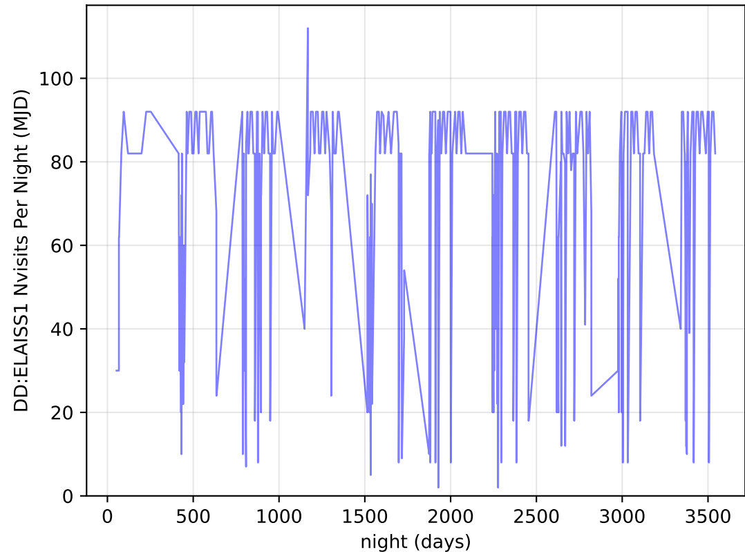
scp_reweight_v3.3_10yrs all bands: DD:ELAISS1 Nvisits Per Night
